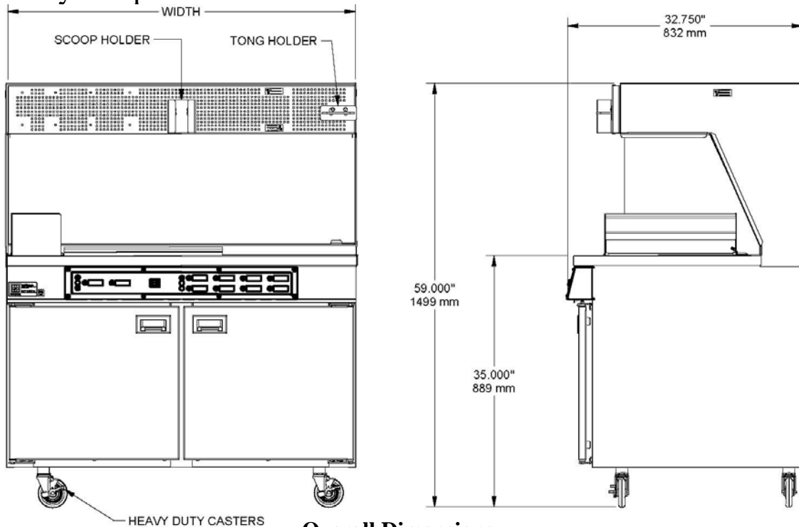
Overall Dimensions Models RR5-48.5 and RR5-42
